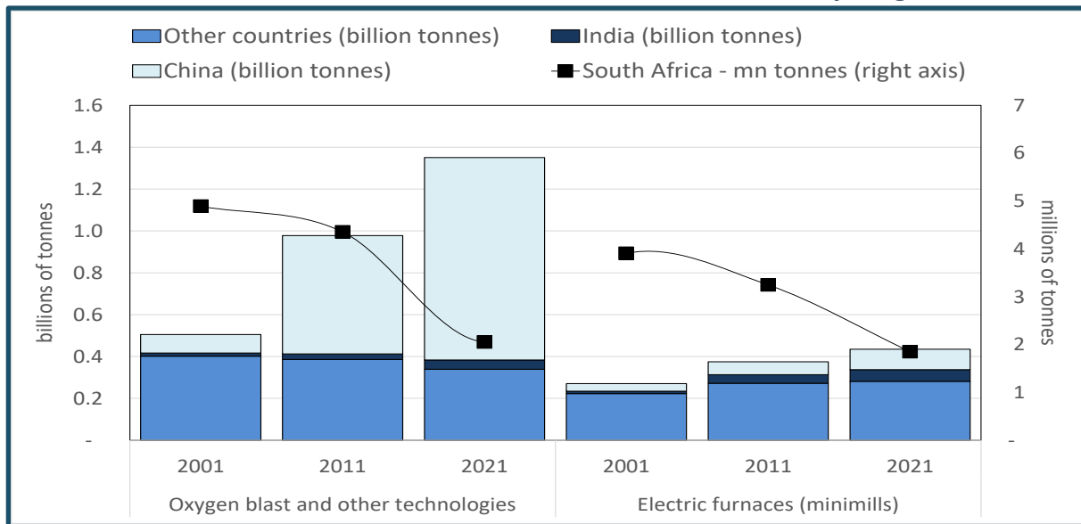
Graph 22. Production of steel by technology type (electric arc furnaces or oxygen blast) for China, India, South Africa and other countries, 2001, 2011 and 2021, by weight
